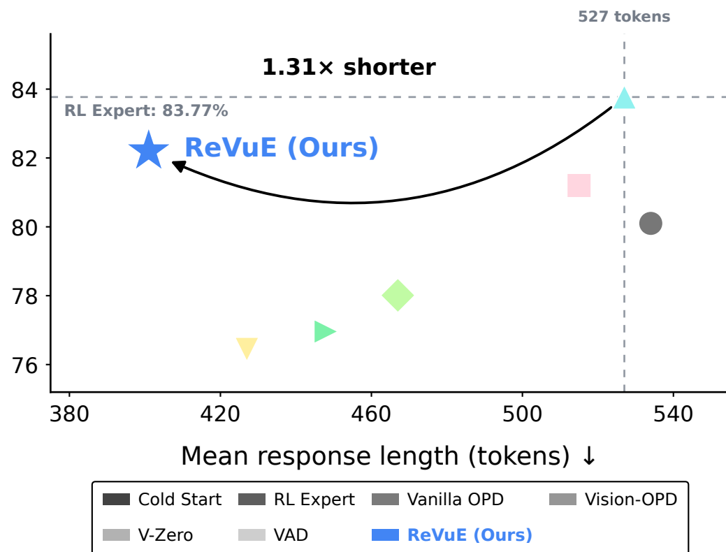
(b) V* Bench
