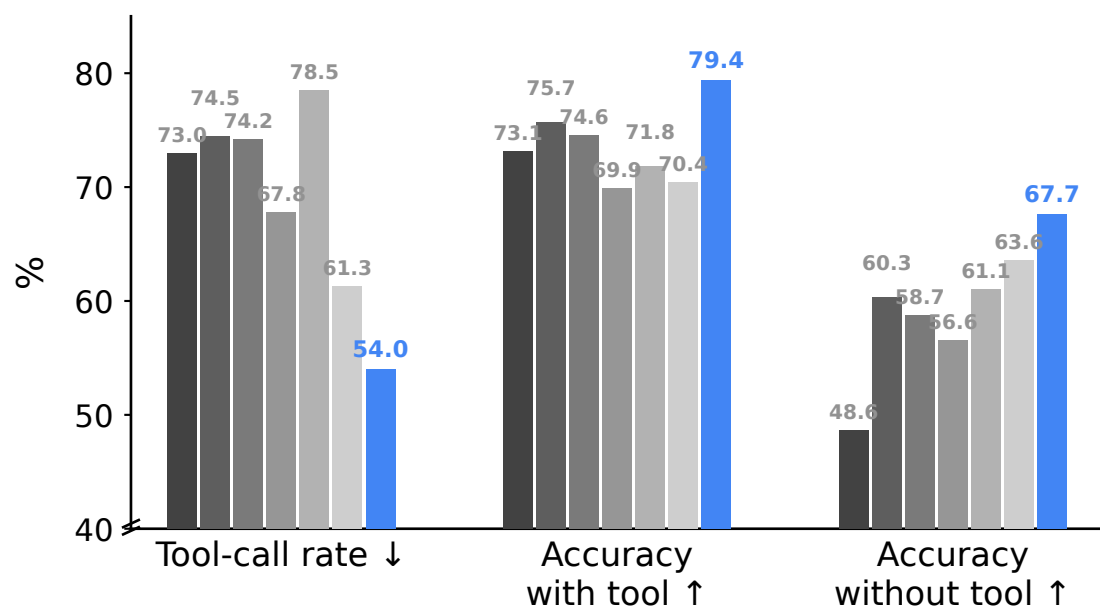
(c) HRBench 8K
