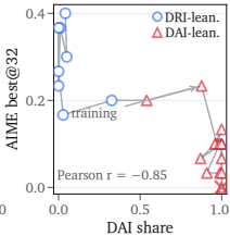
(c) DAI vs. best@32
