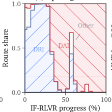
(b) Opening routes
