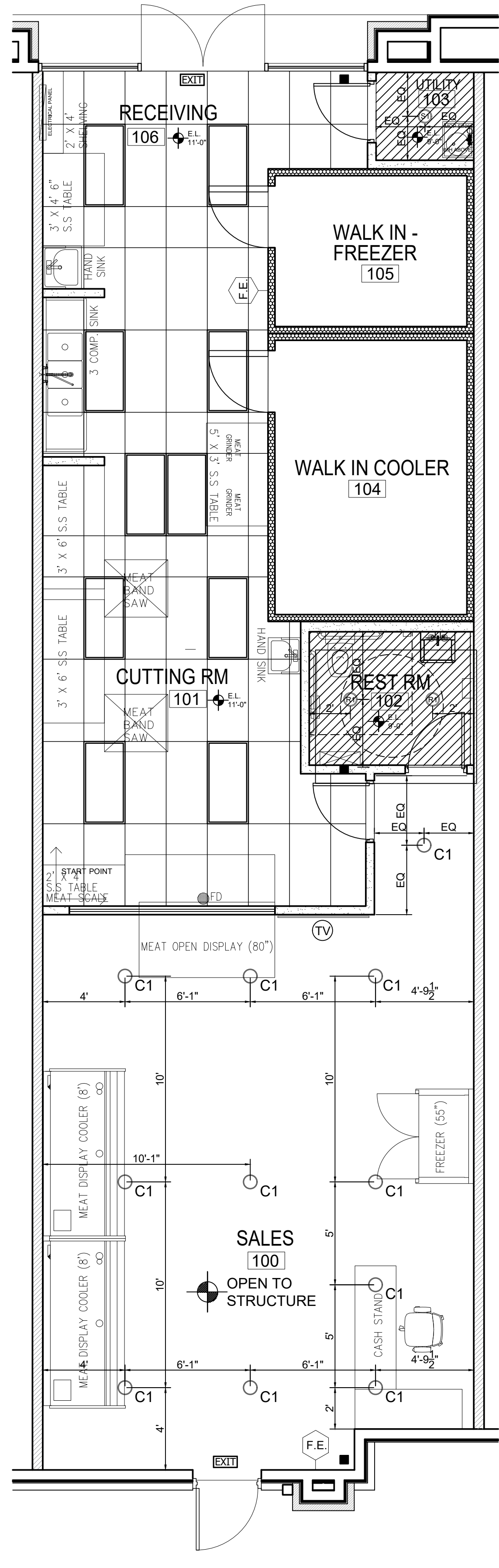
01 REFLECTED CEILING PLAN SCALE: 1/4" = 1'-0"
