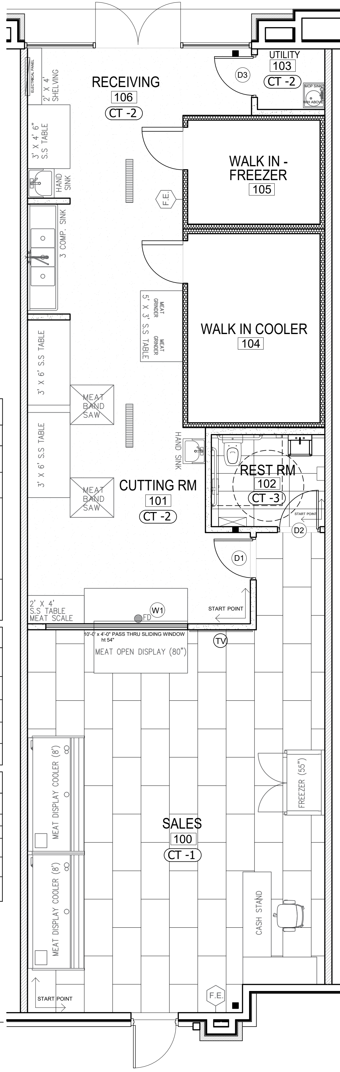
02 RM FINISH PLAN SCALE: 1/4" = 1'-0"
