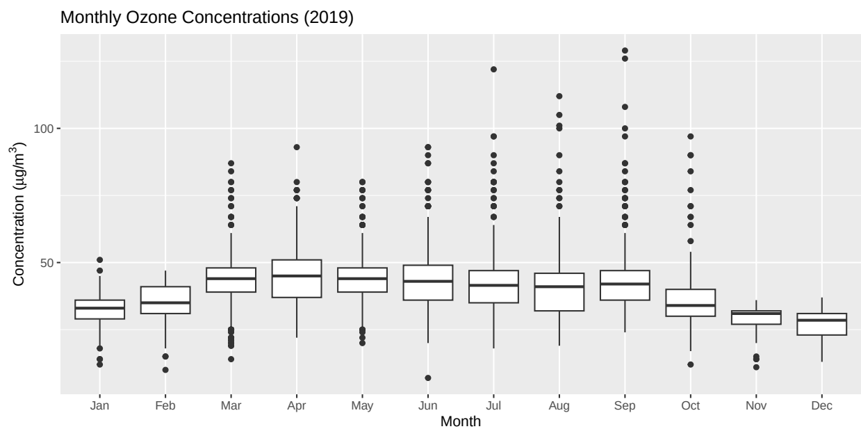
Figure 2: 2019 Monthly Ozone Levels
