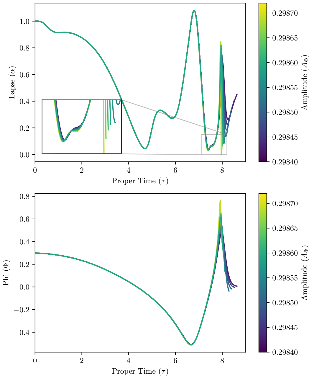
Scalar Field with Superimposed Brill Waves
