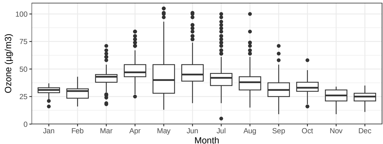
Figure 1: Monthly Ozone (2018).
