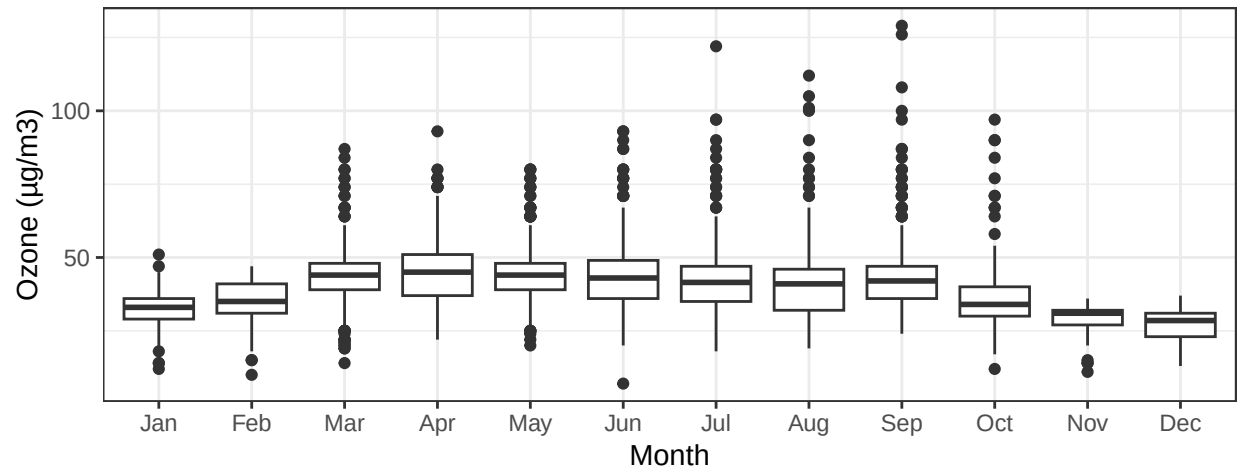
Figure 2: Monthly Ozone (2019).
