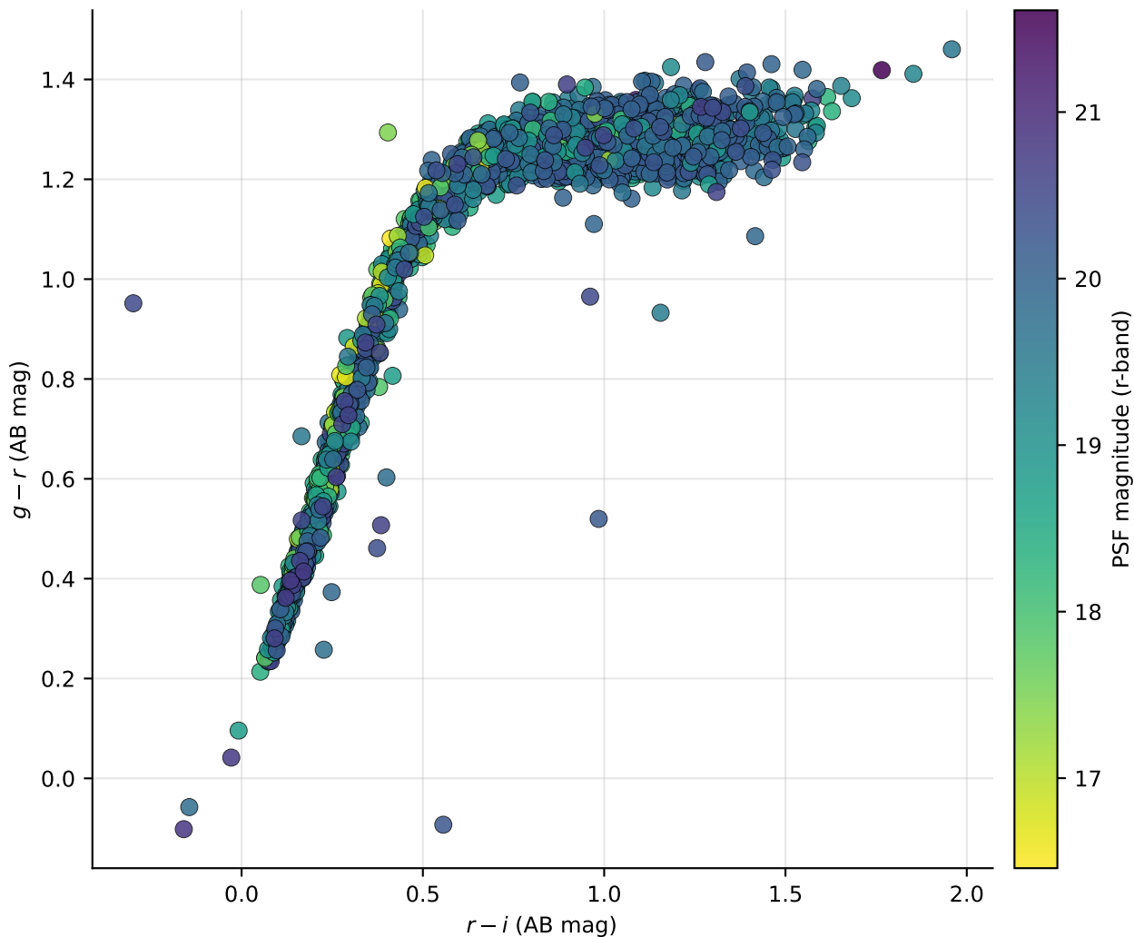
lsst-obj Colour-colour diagram: matched Simbad targets (PSF fluxes, Rubin DP2)
