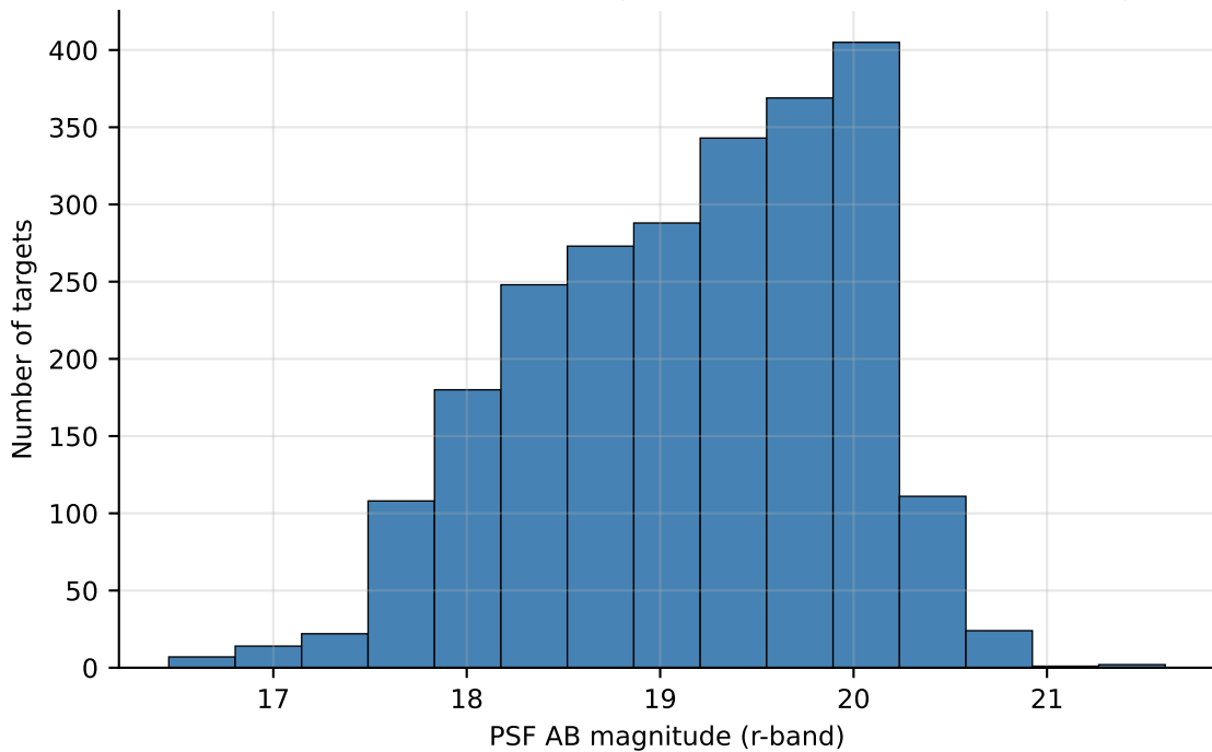
Distribution of r-band PSF magnitudes -- matched Simbad targets
