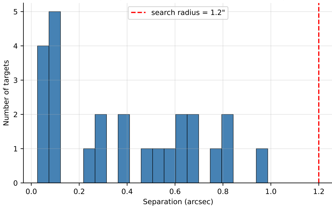
Cross-match separation -- Simbad targets vs LSST objects
