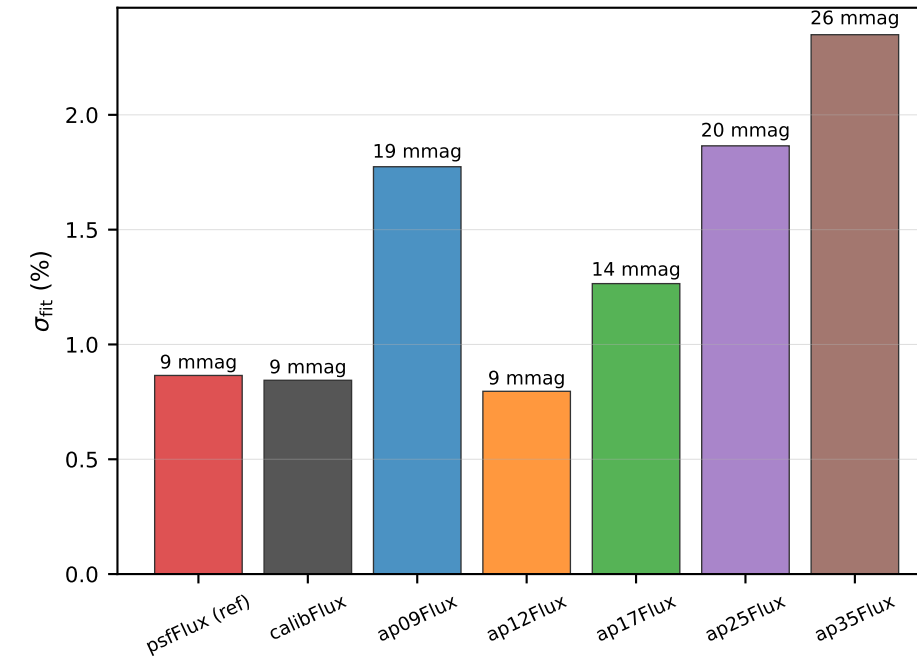
z band
