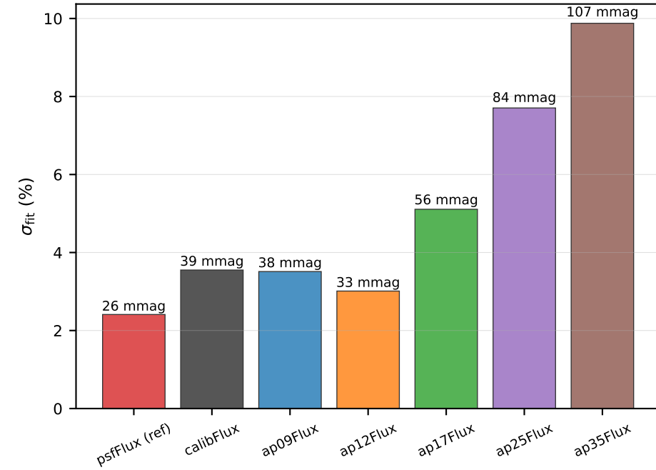
i band
