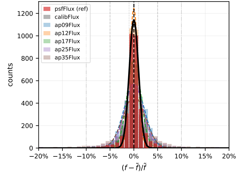
r band
