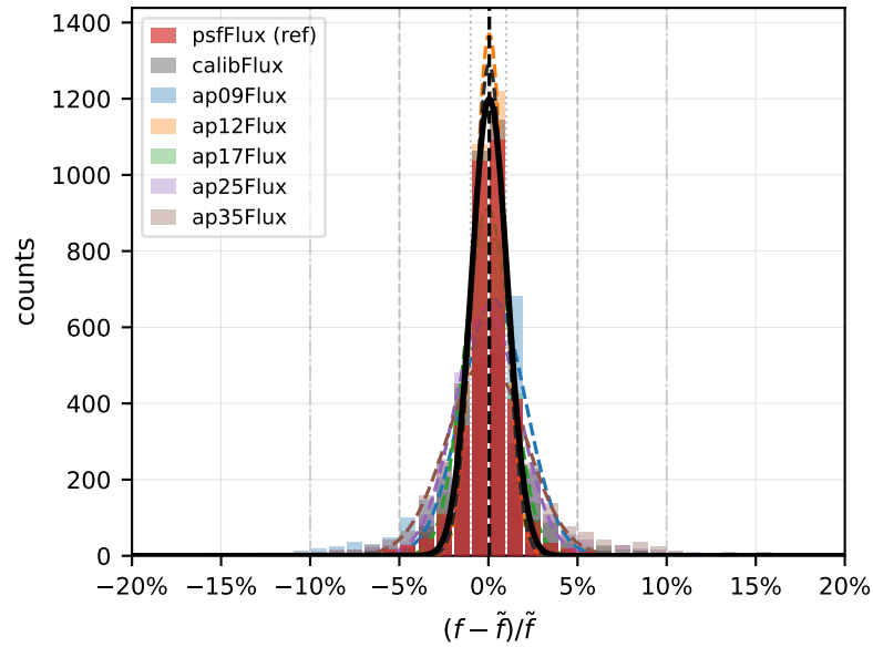
i band
