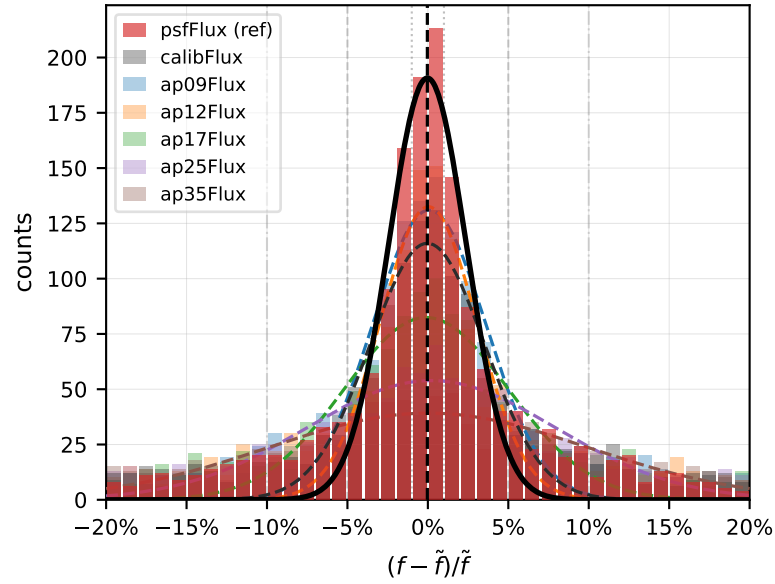
u band
