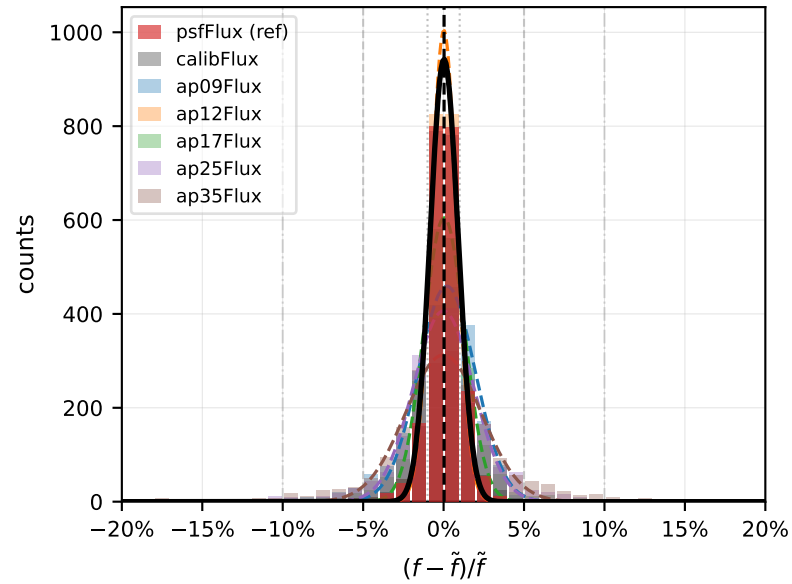
z band
