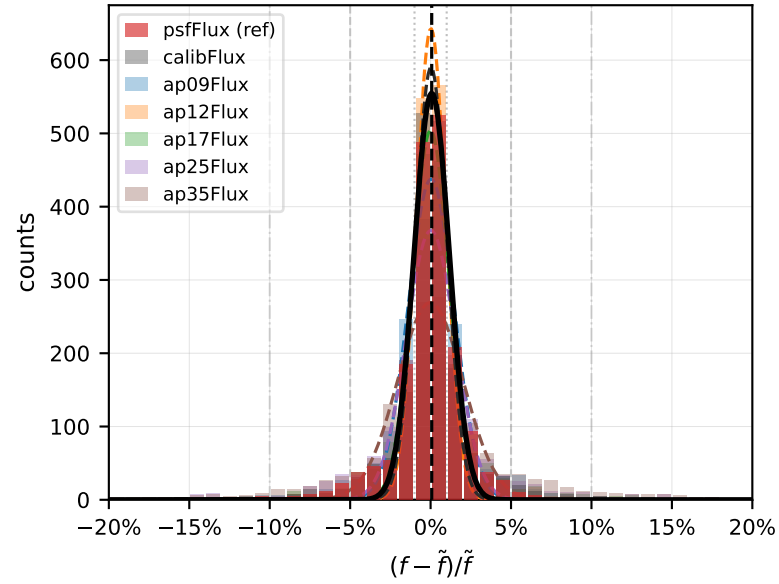
g band
