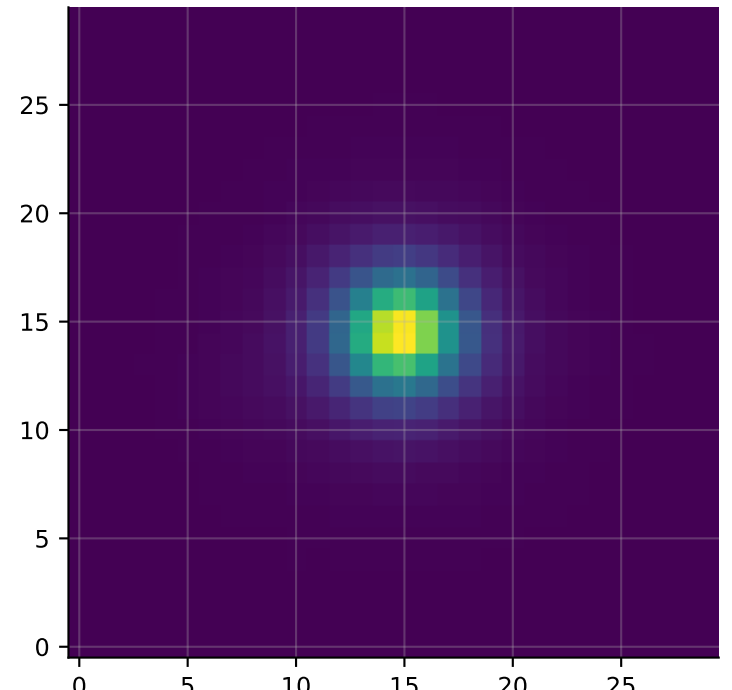
ACS-GC 20099329 (COSMOS,18.9,M1e)
