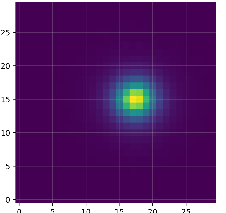
COSMOS 2685690 (COSMOS,19.3,F5)
