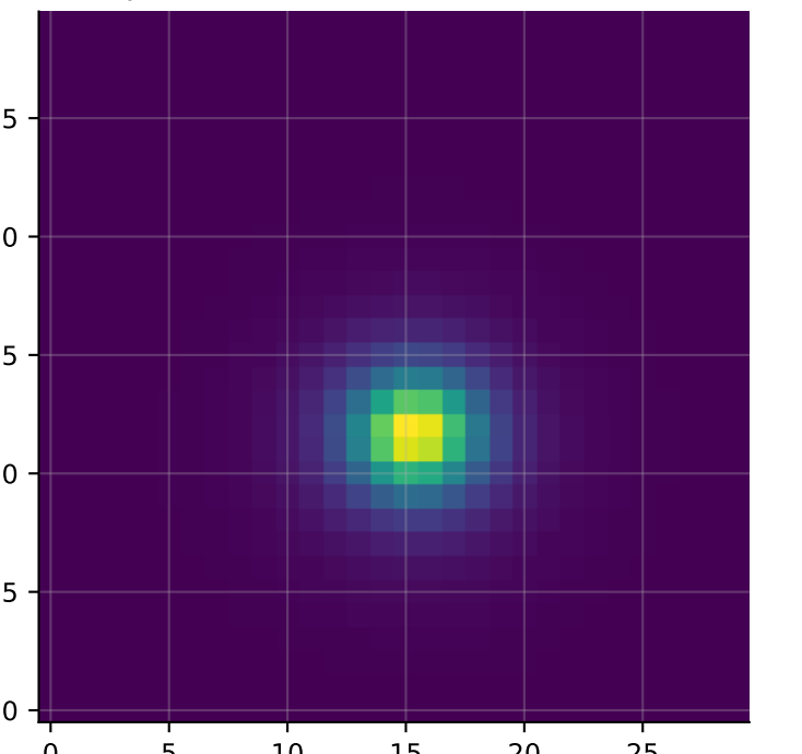
COSMOS 1235283 (COSMOS,19.6,M5)
