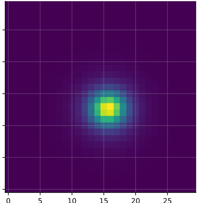
COSMOS 2804135 (COSMOS,18.5,F5)
