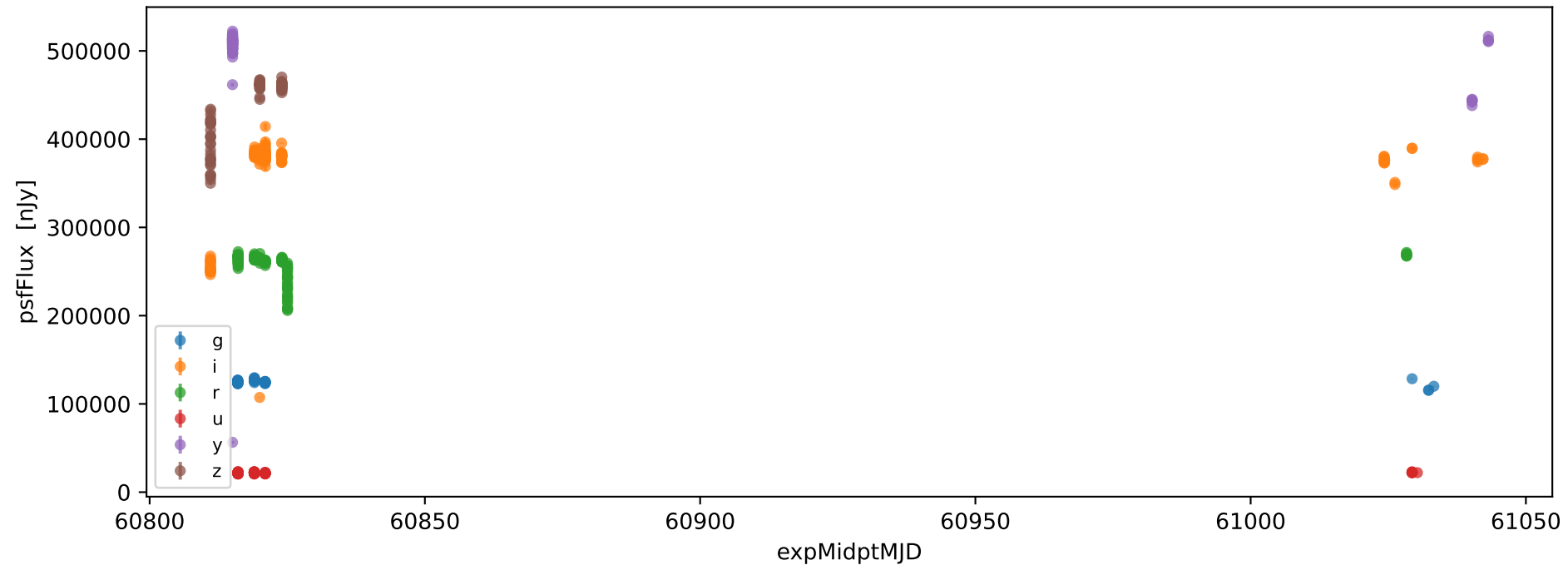
Light curve (demo) — 2MASS J09595063+0223163
