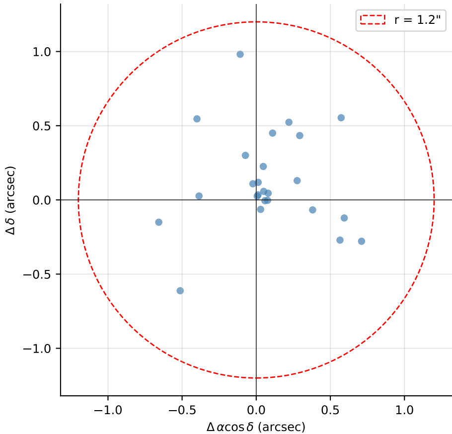
Positional offsets: Simbad - LSST
