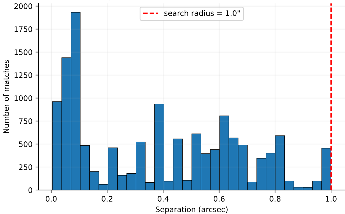
Cross-match separation - Simbad targets vs LSST sources (all visits)
