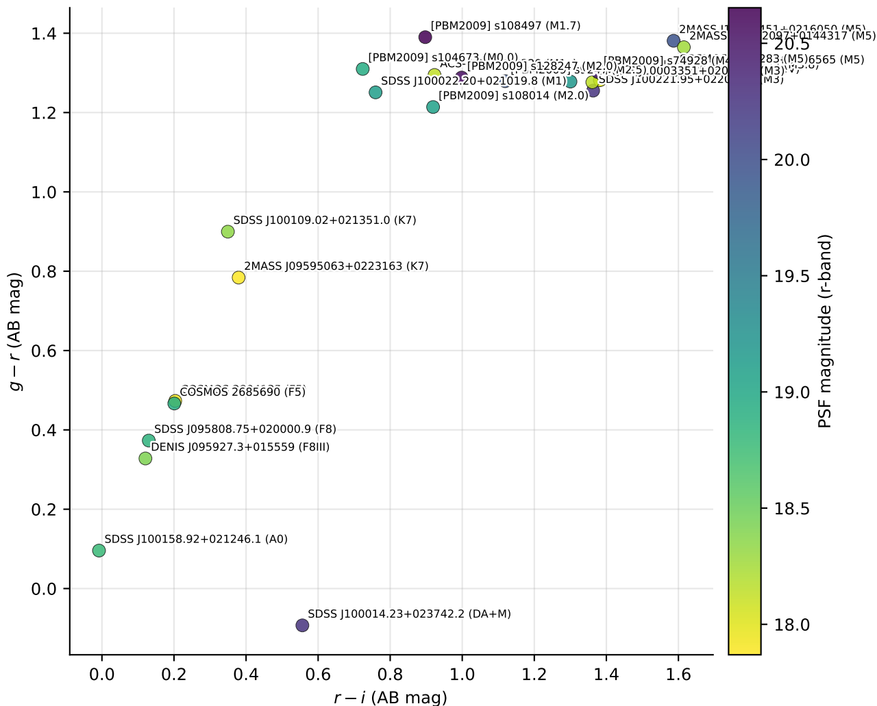
Isst-obj Colour-colour diagram: matched Simbad targets (PSF fluxes, Rubin DP2)
