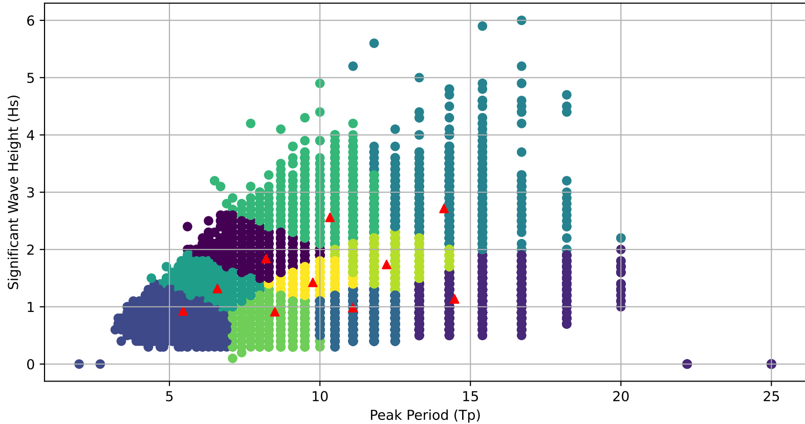
Wave Data Clustering for SJPR Buoy
