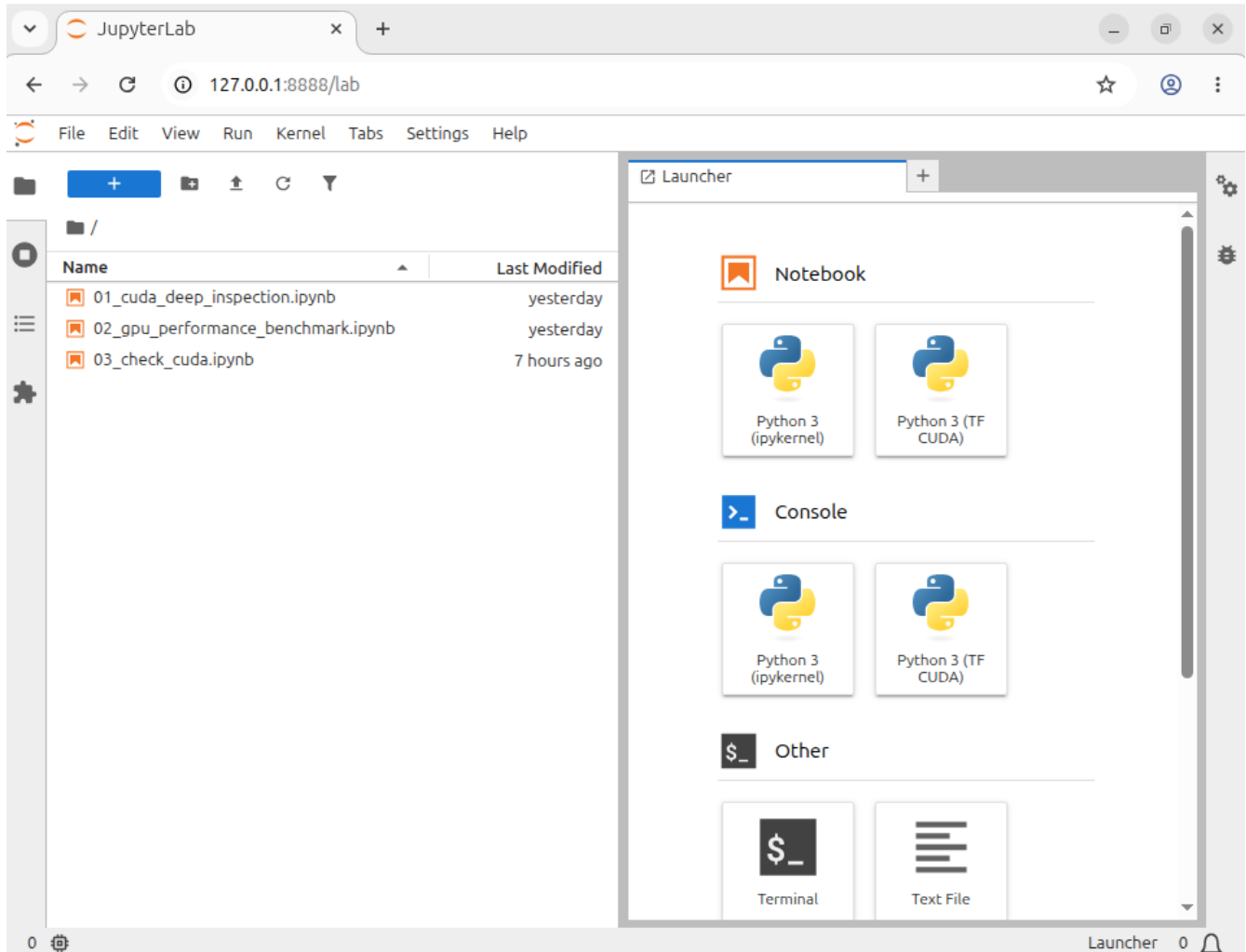
Figure 3.3-1 JupyterLab Startup
