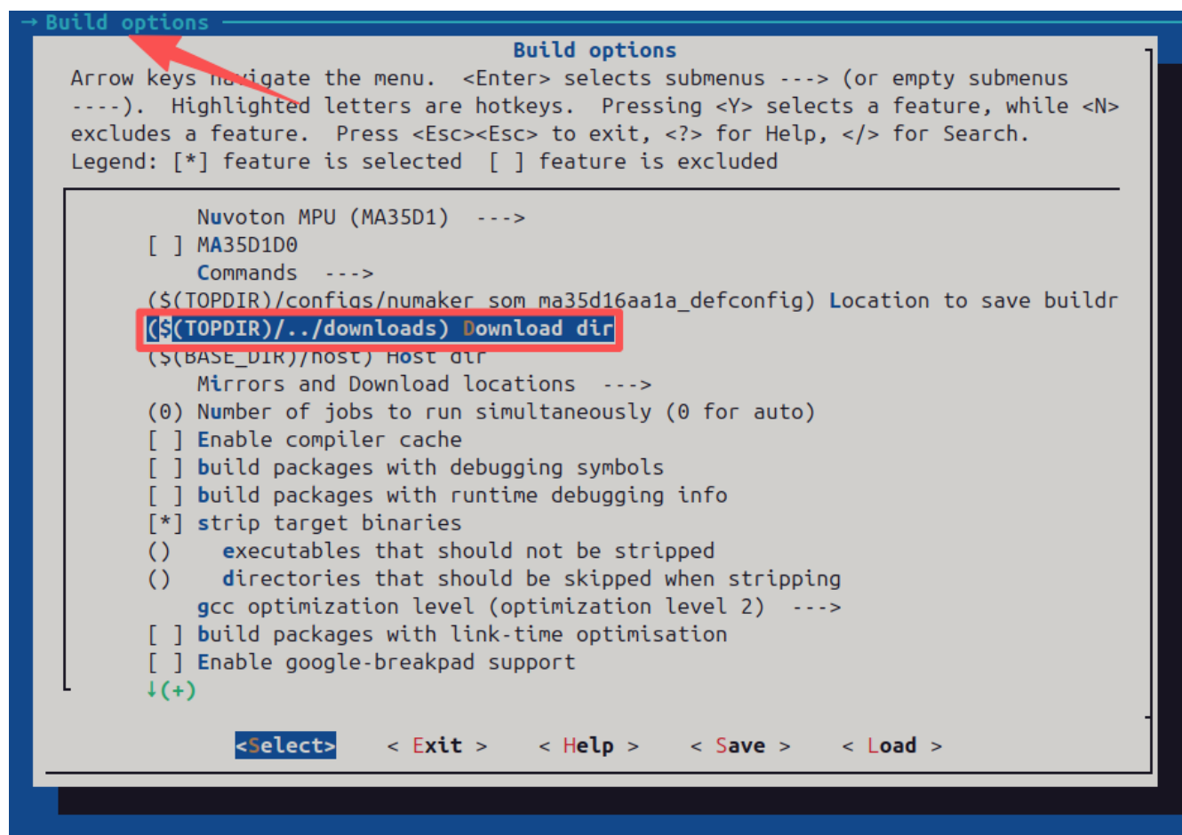
Figure 2.3.1-1 Download dir
