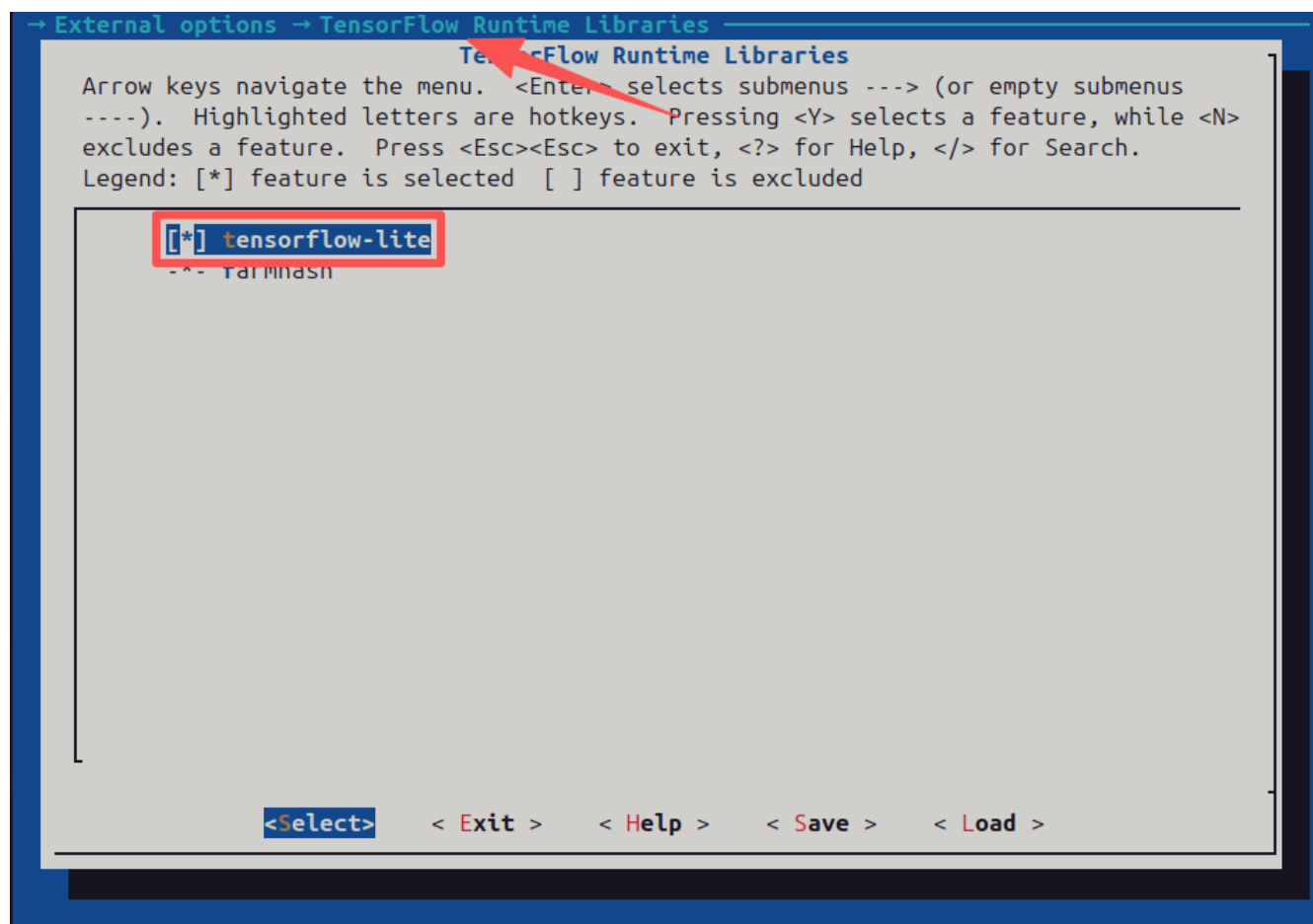
Figure 2.3.3-1 tensorflow-lite package
