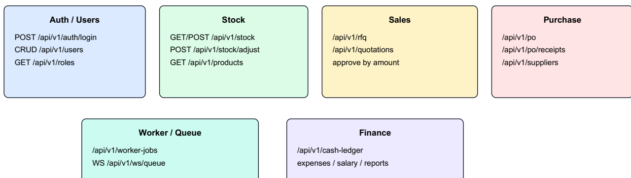
RBWF API Design Overview
