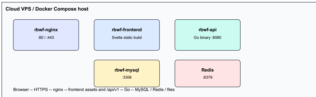
RBWF Deployment Diagram
