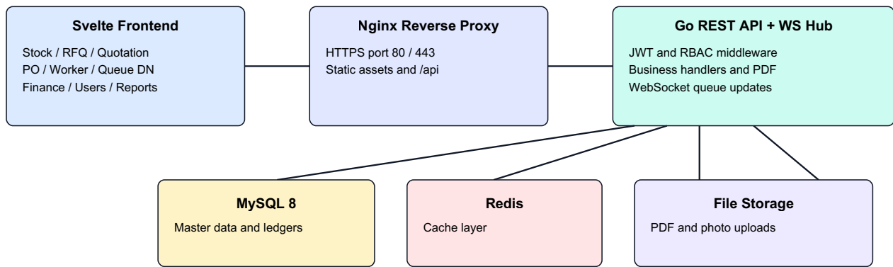
RBWF Component Diagram
