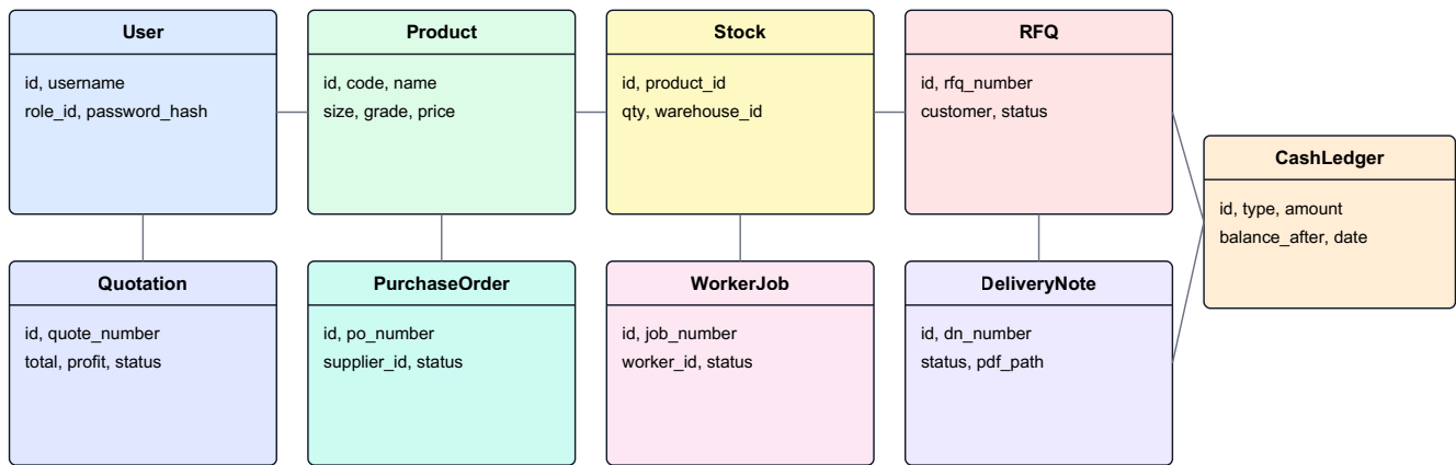
RBWF Class Diagram (domain)
