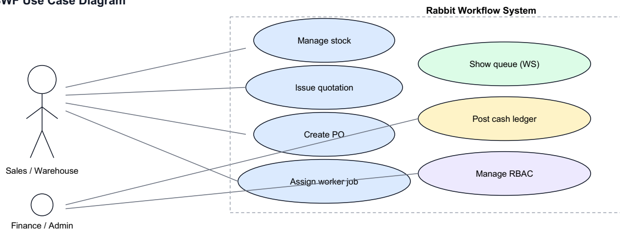
RBWF Use Case Diagram
