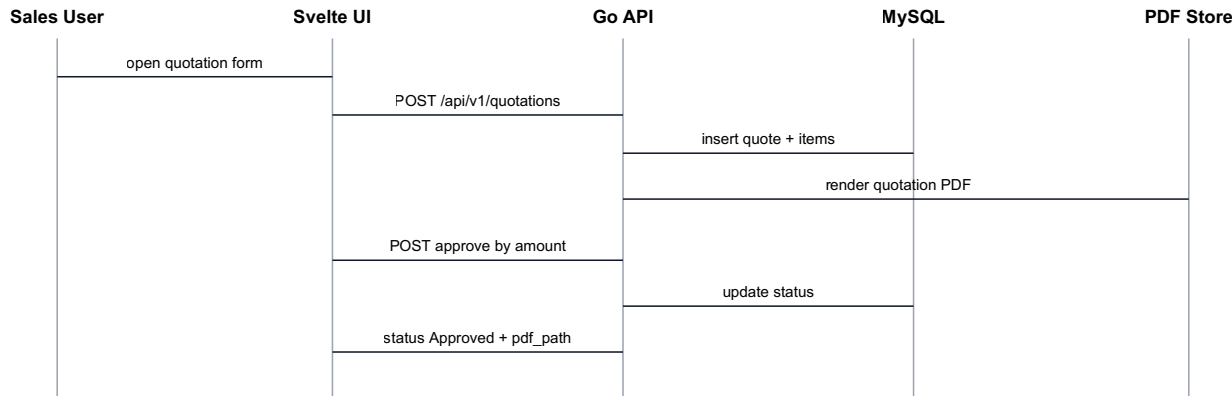
Sequence: create and approve quotation
