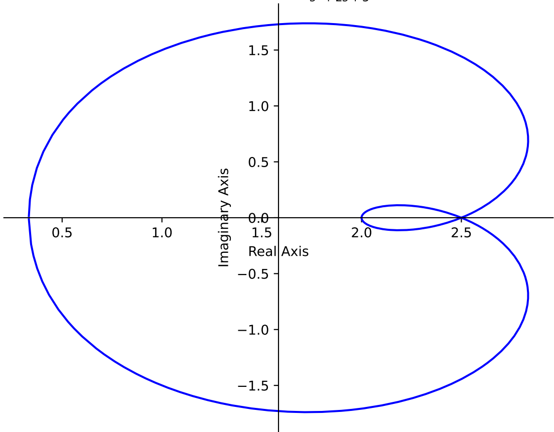
Nyquist Plot of \frac{2s^2 + 5s + 1}{s^2 + 2s + 3}
