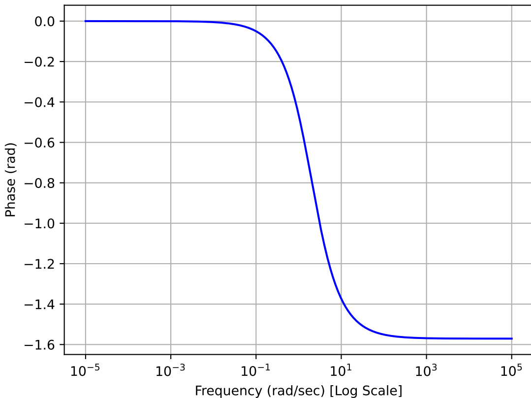
Bode Plot (Phase) of \frac{1}{s+2}
