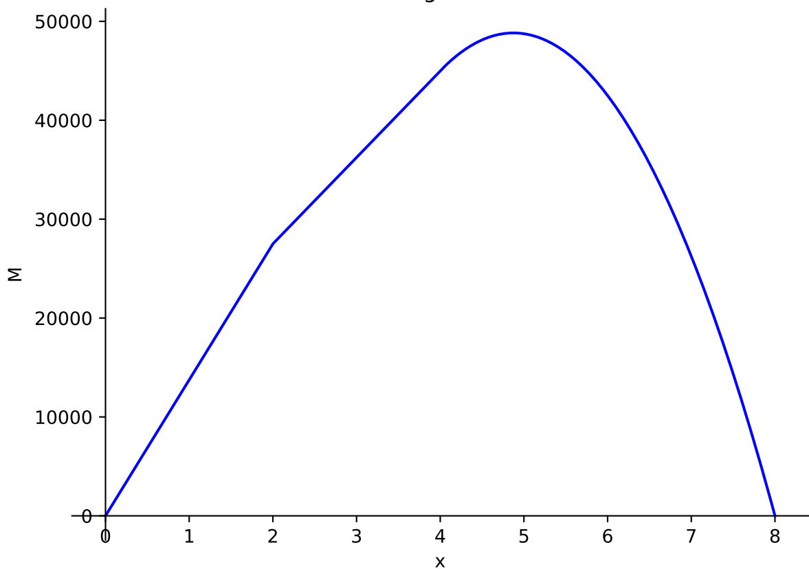
Bending Moment
