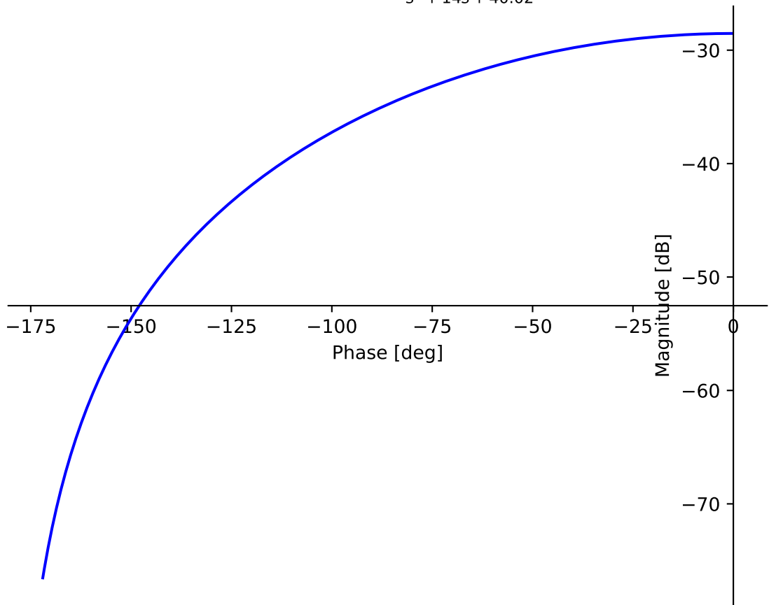
Nichols Plot of \frac{1.5}{s^2 + 14s + 40.02}
