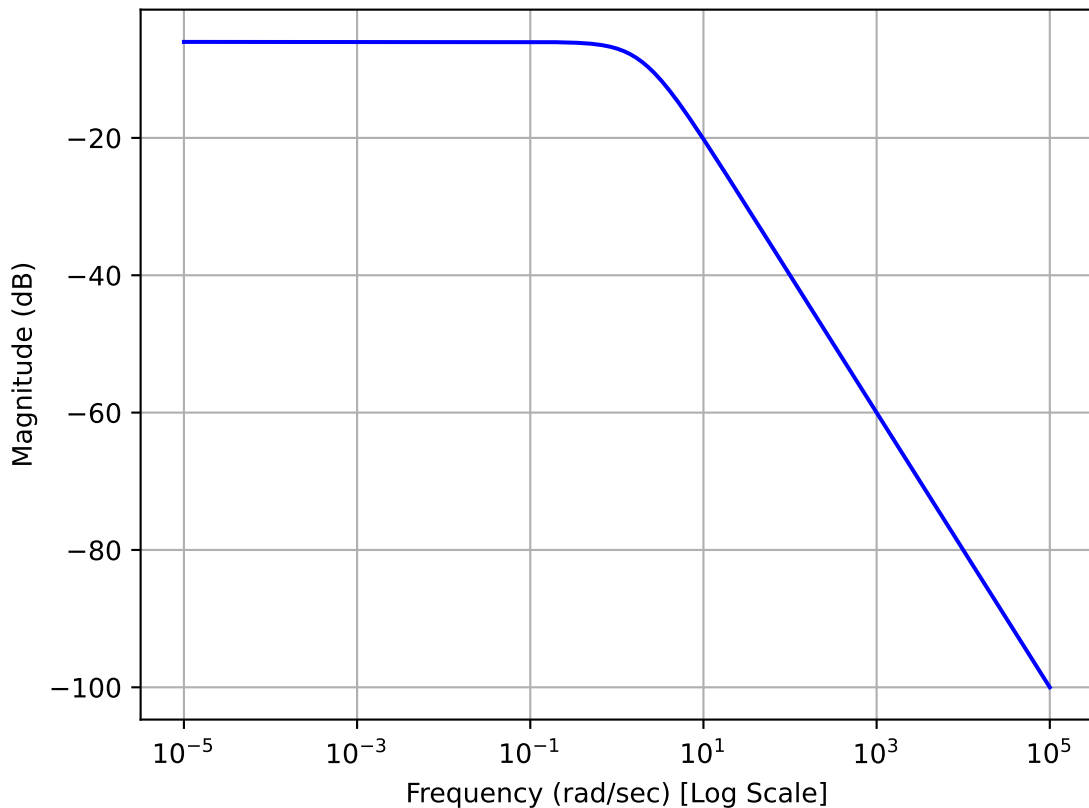
Bode Plot (Magnitude) of \frac{1}{s+2}
