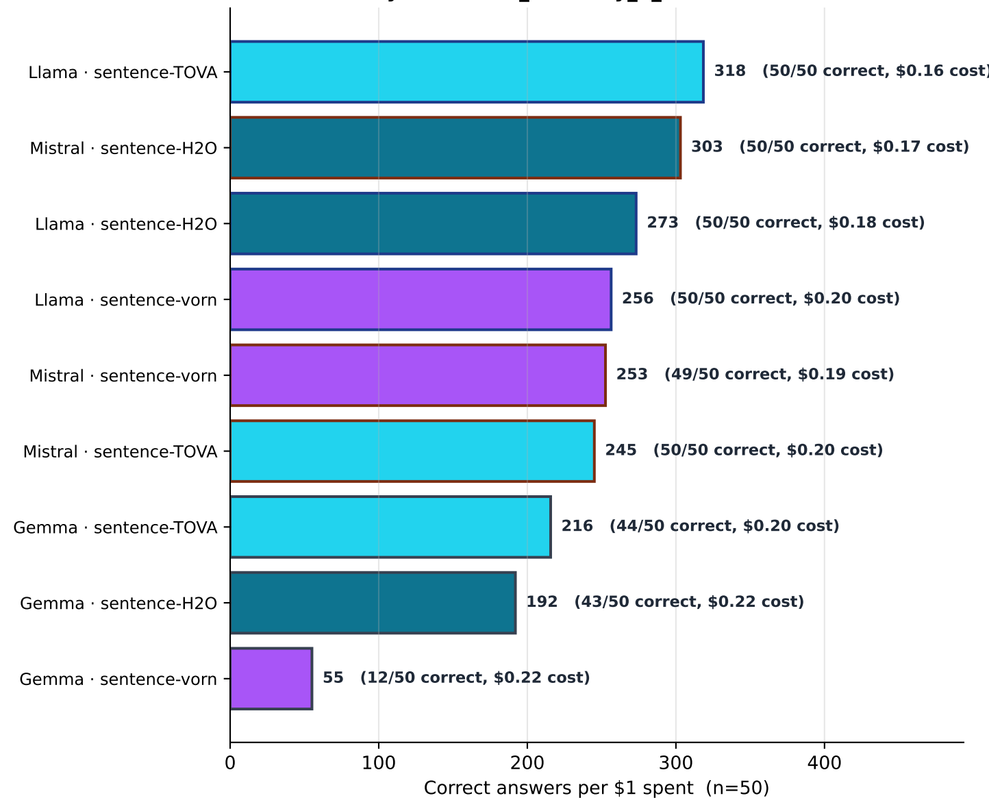
Primary task: niah_multikey_1_4k (B=1024, n=50)
