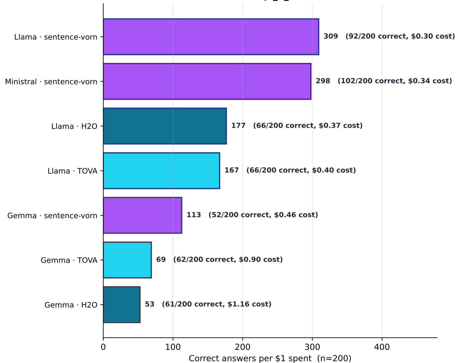
Cross-task validation: qa_2_4k (B=1024, n=200)
