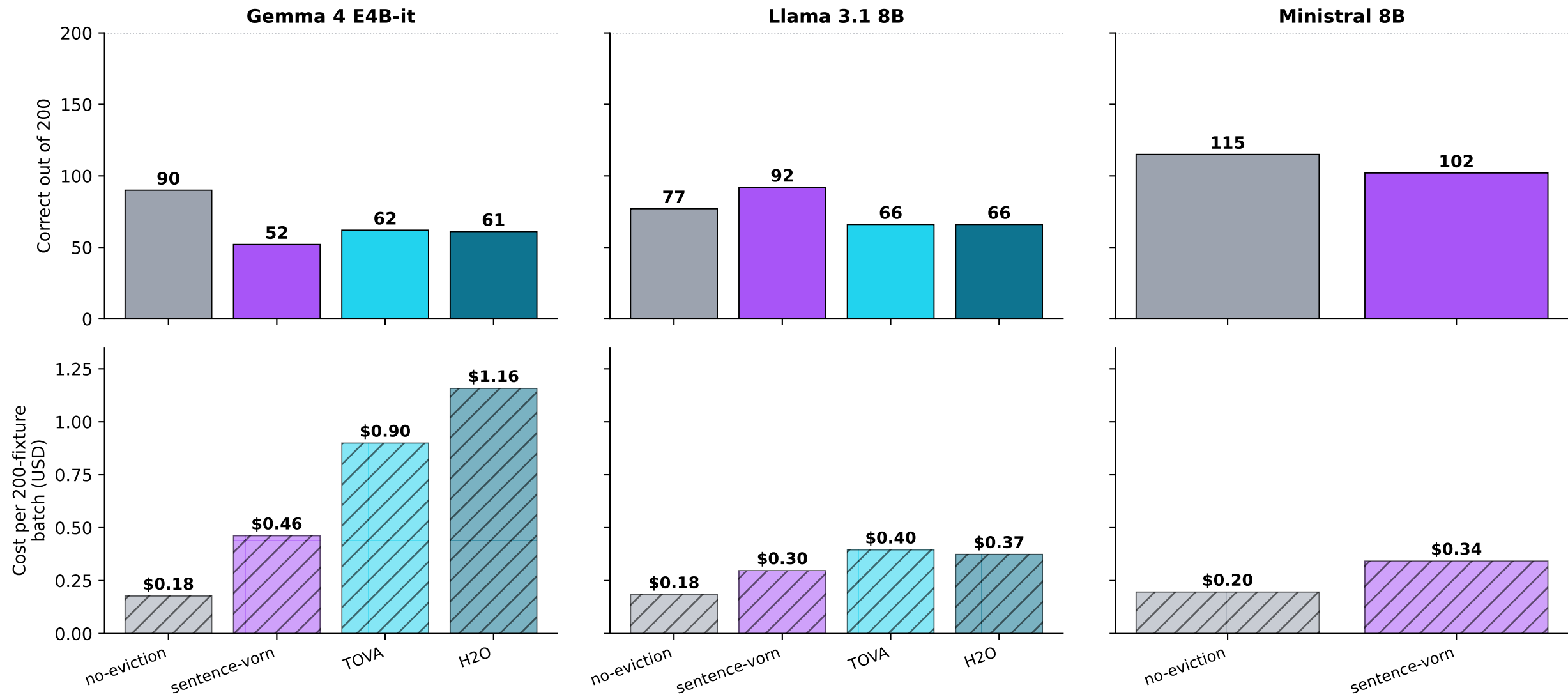
Variant A — Anchored bars: raw correct-out-of-200 on top, raw cost on bottom, by family
