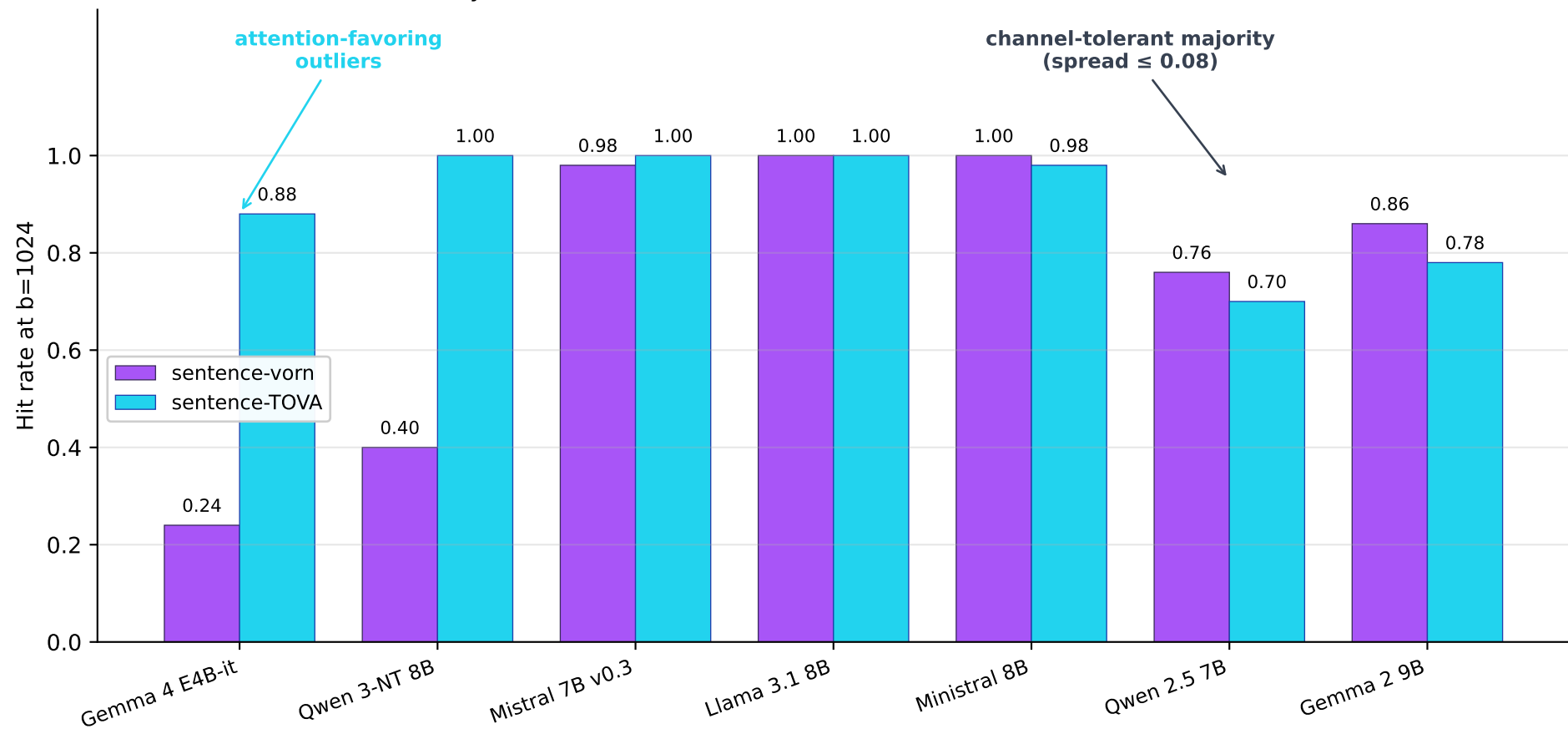
Cross-family channel-favoritism axis: sentence-vorn vs sentence-TOVA at b=1024
