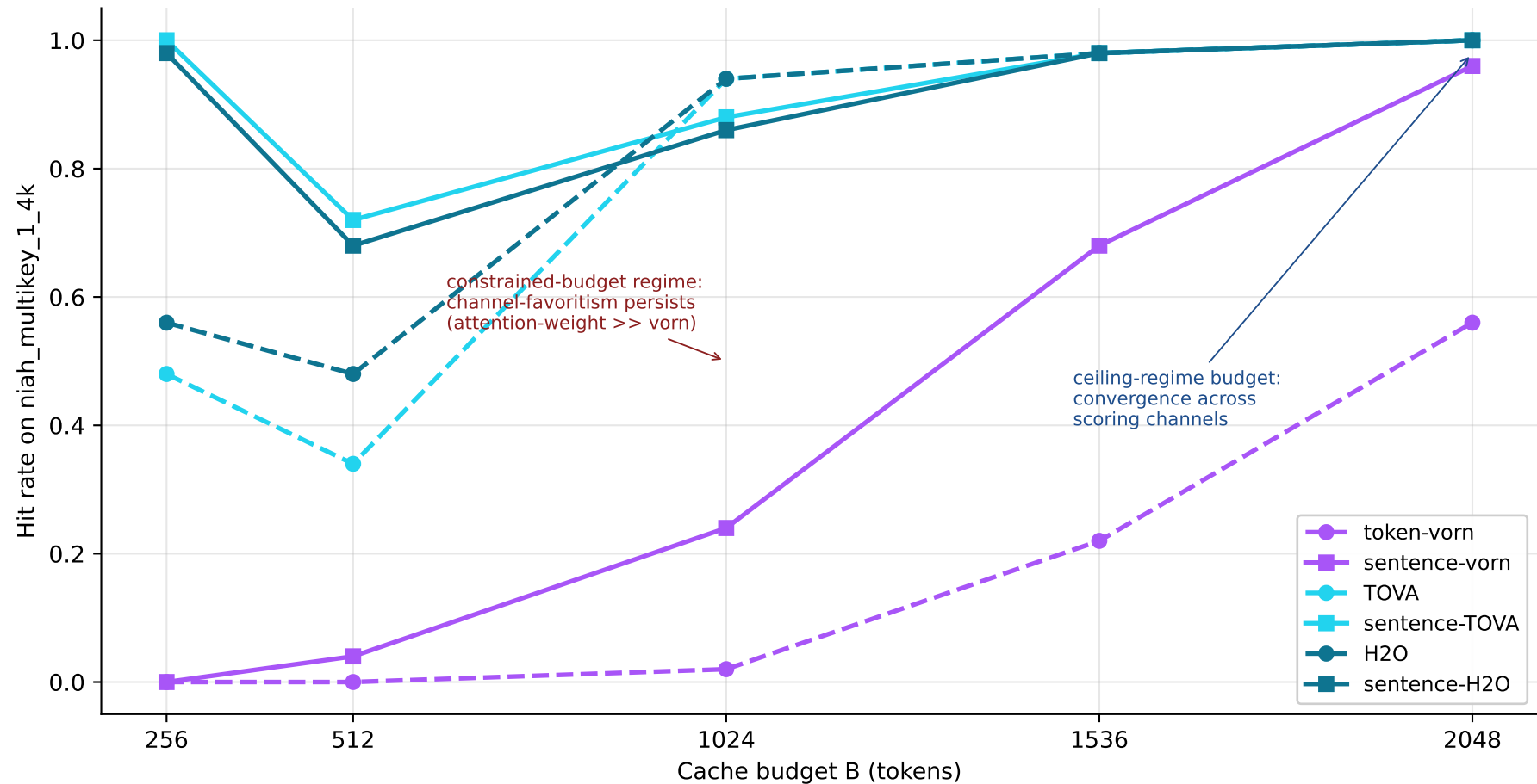
Gemma 4 E4B-it: budget-sweep degradation curve at 4k context
