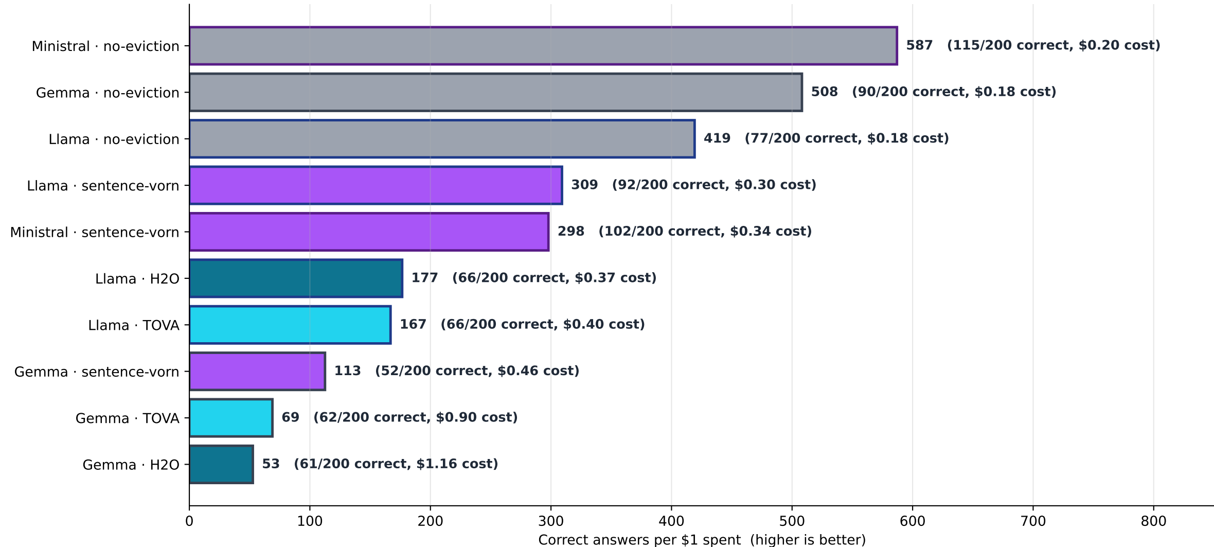
Variant D — Correct-per-$1 leaderboard (rank-ordered); raw correct \& cost shown to the right
