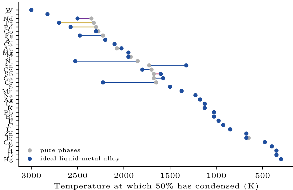
Effect of alloying on the condensation ladder
