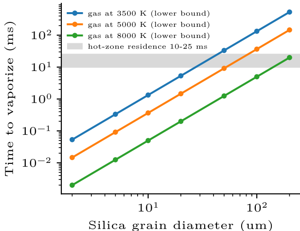
Mineral grains: time grows as d^2
