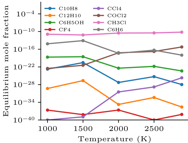
Complex molecules left at equilibrium
