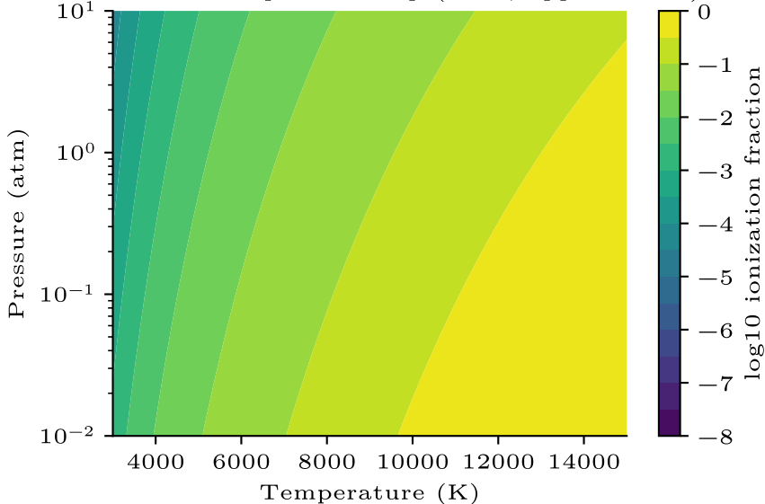
Ionization of the plasma heap (Saha, upper bound)
