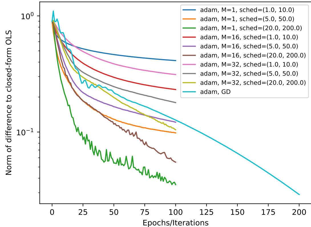
SGD vs GD of adam for OLS
