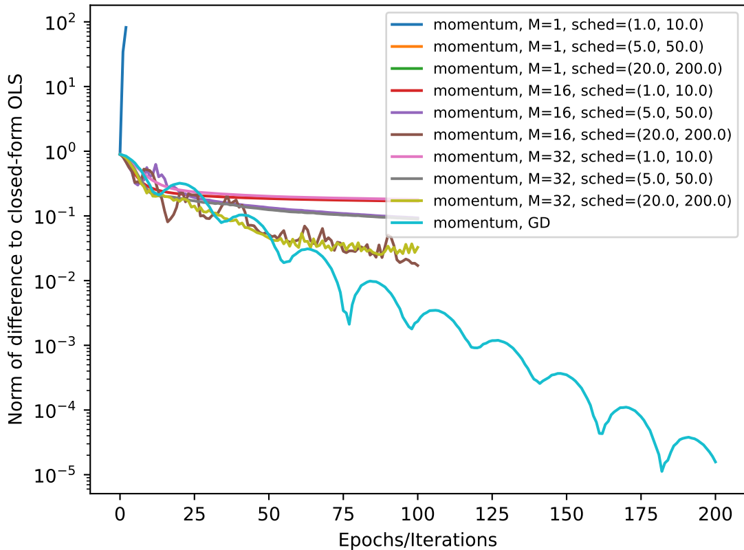
SGD vs GD of momentum for OLS
