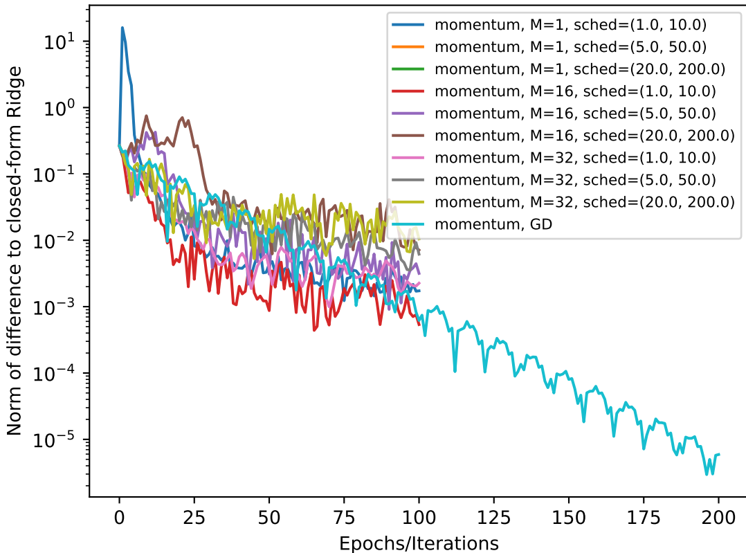
SGD vs GD of momentum for Ridge
