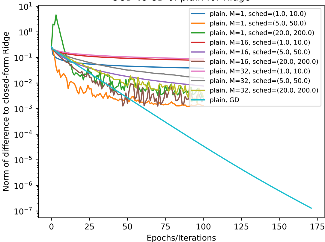
SGD vs GD of plain for Ridge
