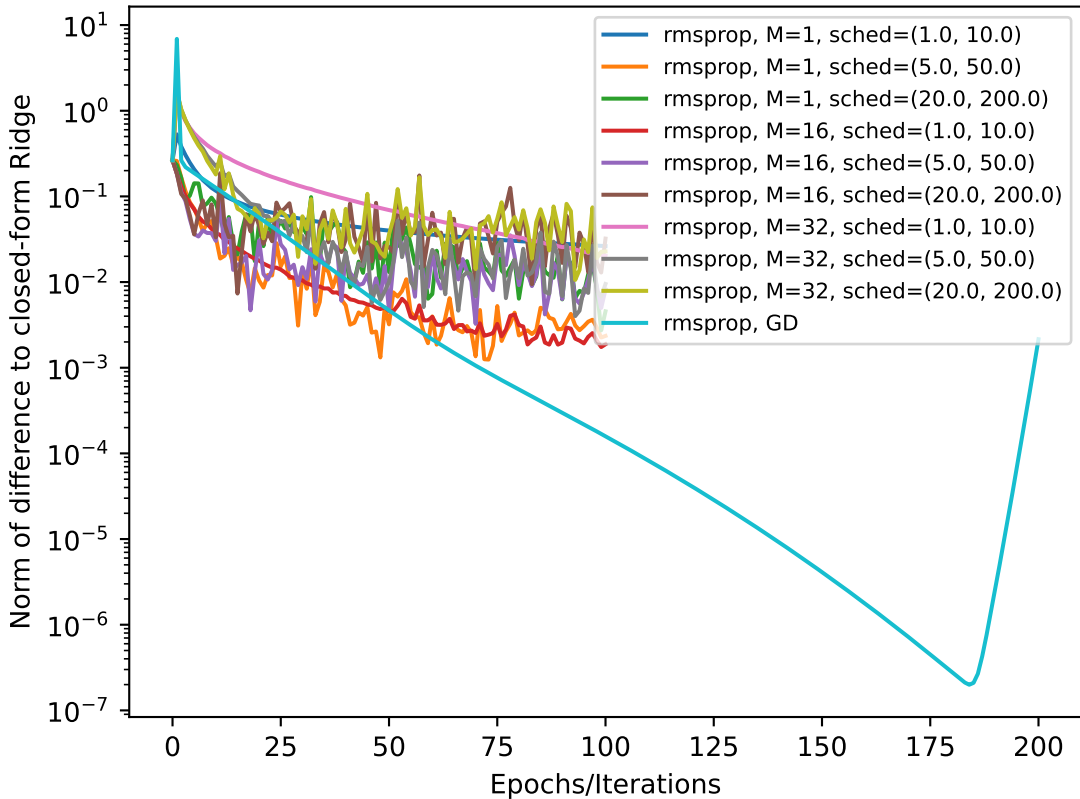
SGD vs GD of rmsprop for Ridge
