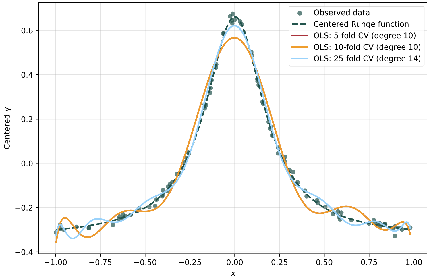
OLS Estimates of the Runge Function
