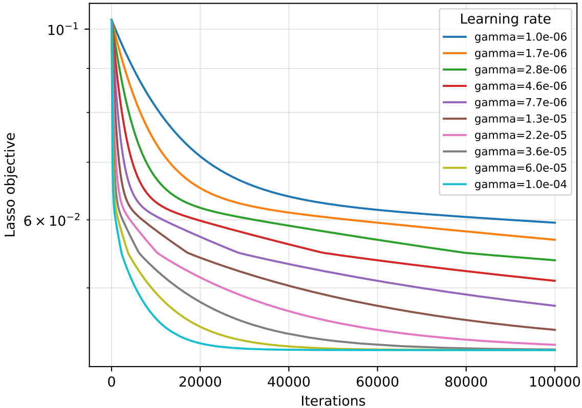
Lasso convergence: momentum
