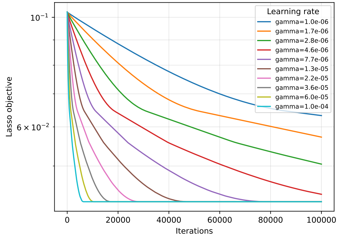
Lasso convergence: rmsprop
