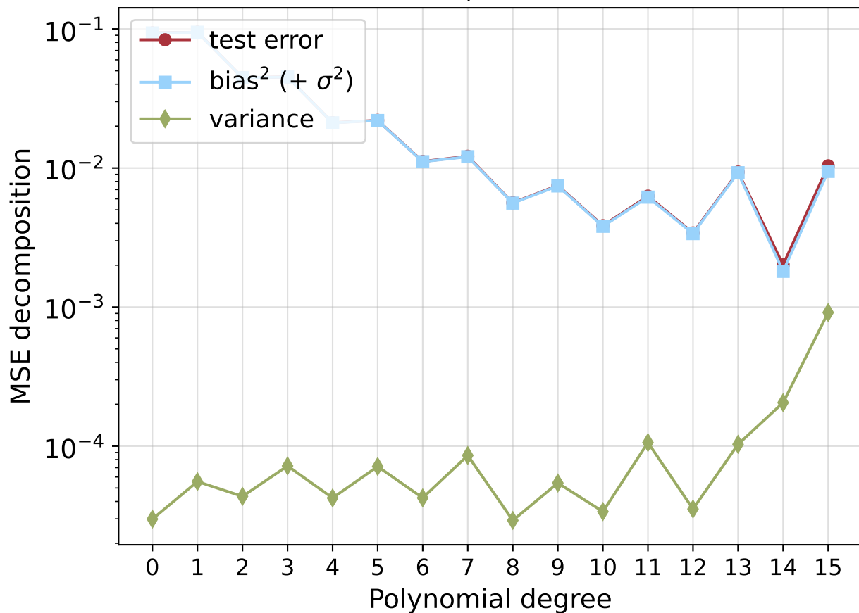
OLS MSE Decomposition (25-Fold CV)
