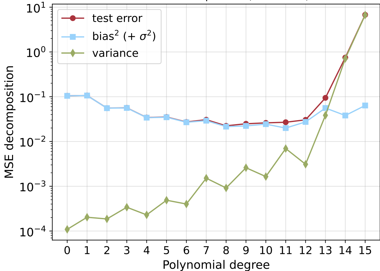
OLS MSE Decomposition (10-Fold CV)
