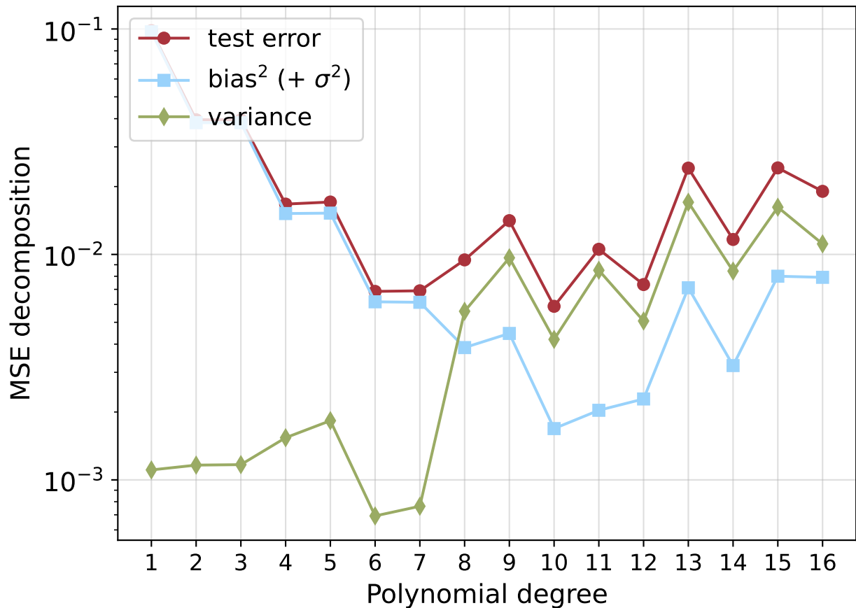
Lasso MSE Decomposition (5-Fold CV)
