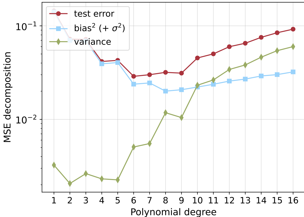
Ridge MSE Decomposition (5-Fold CV)
