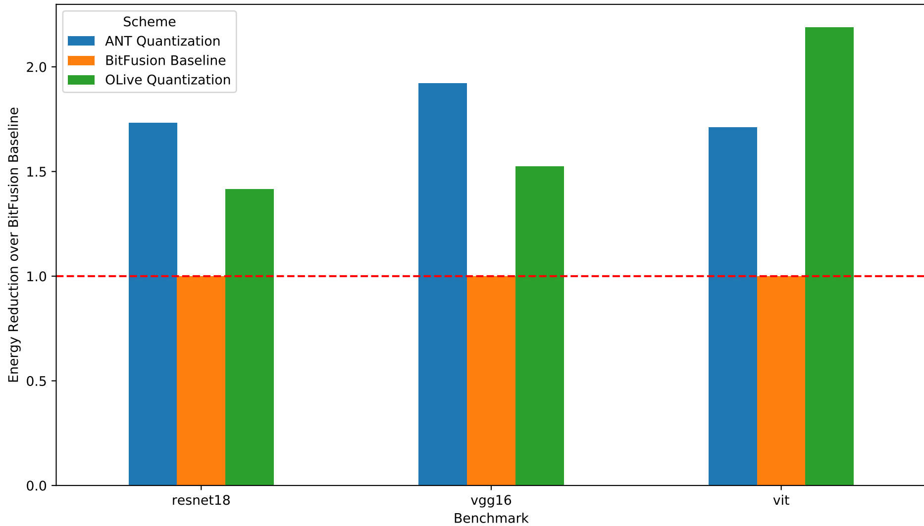
Quantization Schemes Energy Comparison
