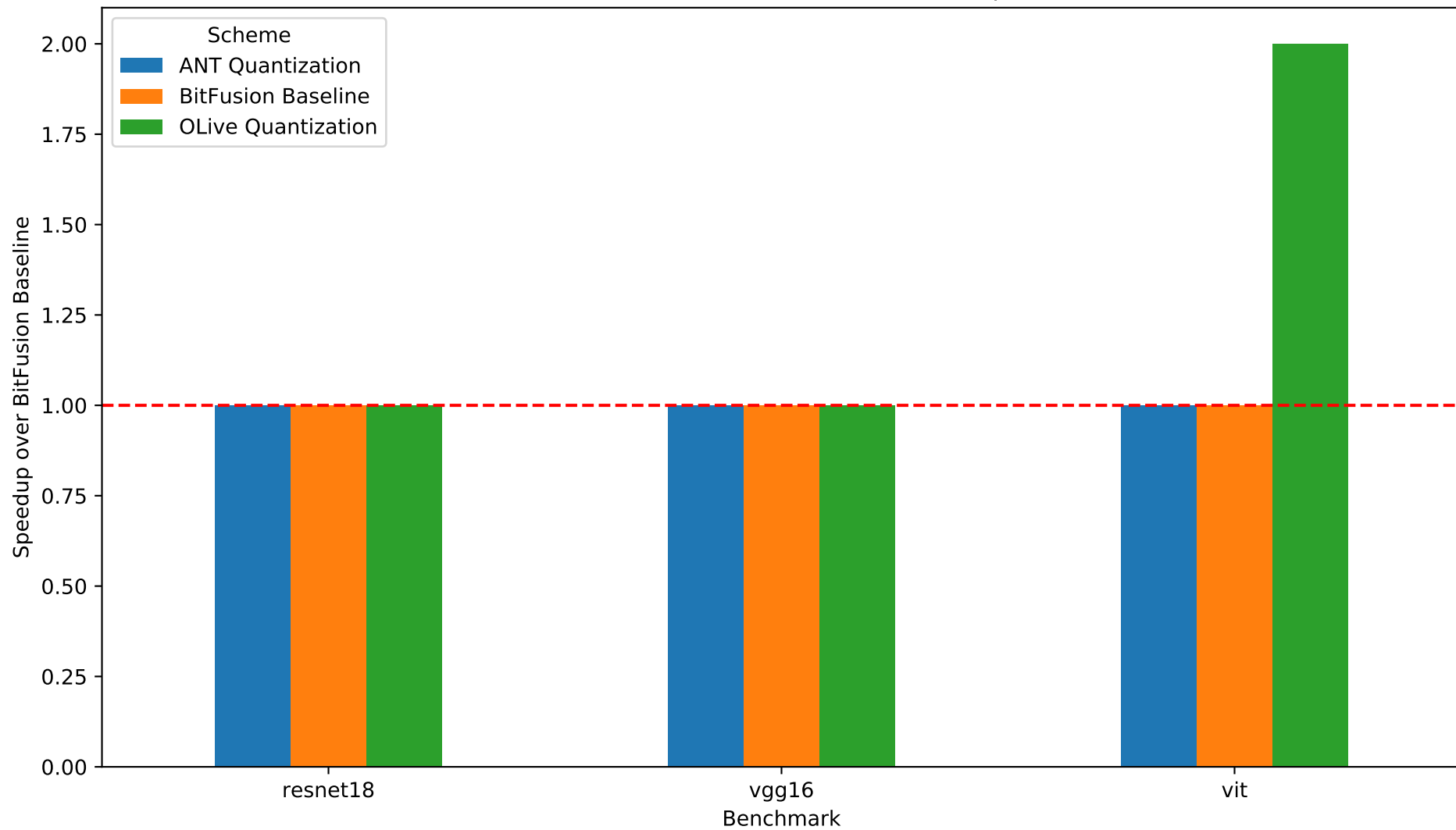
Quantization Schemes Performance Comparison
