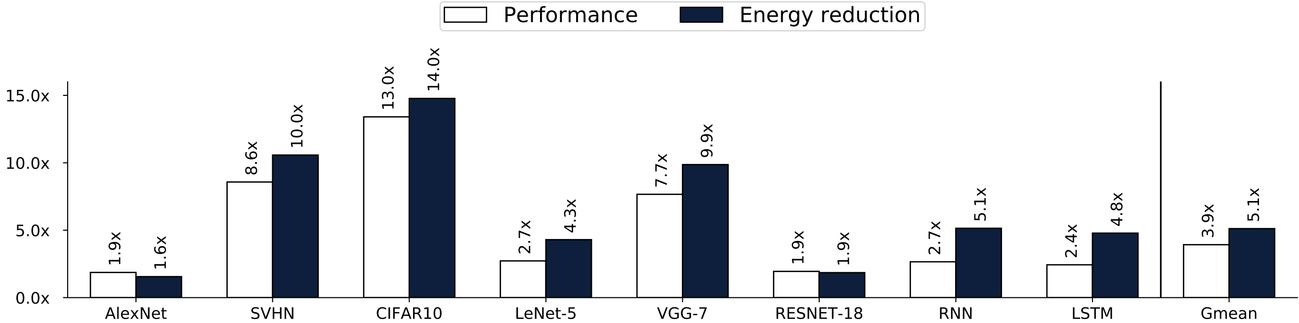
Performance-over-Eyeriss
