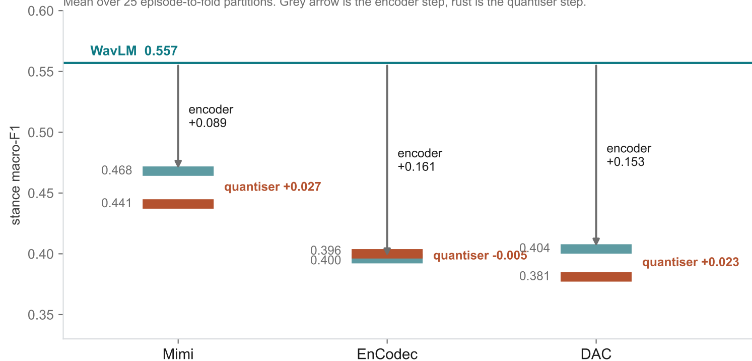
Figure 4.1 The encoder step is 3.3 times the quantiser step in Mimi and 6.7 times in DAC. In EnCodec the quantiser costs nothing measurable.
