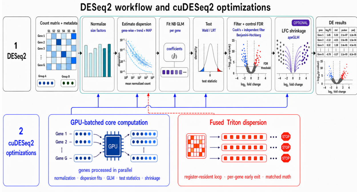
Figure 1: Overview of cuDESeq2. Top , the five stages of a DESeq2 run. Bottom , where the GPU work goes: DESeq2’s per-gene, sequential CPU work (dispersion estimation, the negative-binomial GLM, and apeGLM LFC shrinkage) is batched across all genes ( left , solid arrows), and the dispersion fit, which is limited mainly by launch latency, has a fully fused Triton implementation ( right , dashed arrow). A third mode uses CUDA-graph chunked replay; the three modes are compared in Table 1. Every stage is checked against R DESeq2 step by step (Sec. 3.2).
